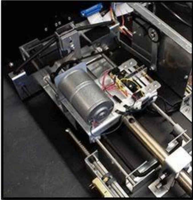
AV-IFR MECHANISM WITH SERVO MOTOR ELEVATOR TRIM
